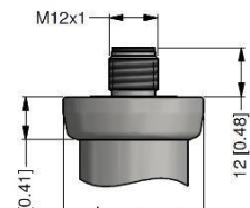
M12x1 4-pin (IP 67)
